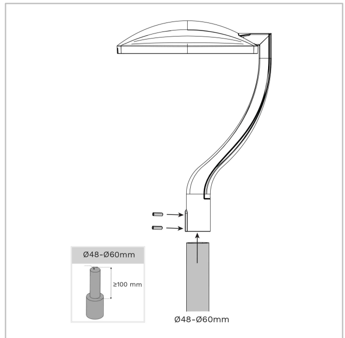
TOPIA | Dedicated bracket for post-top mounting on Ø48-Ø60mm spigots - 2xM8 screws
