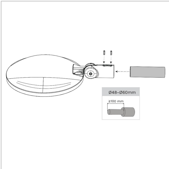
TOPIA | Universal slip-over mounting for Ø48-60mm spigots - 2xM8 screws
